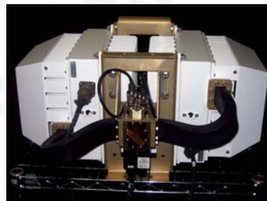
80 - 125W C-Band 1+1
